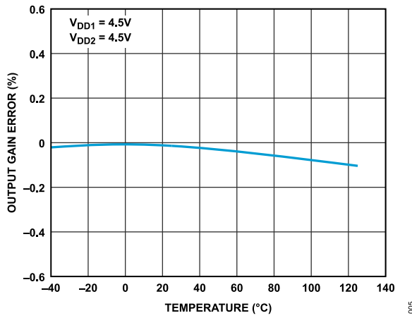
Figure 5. Output Gain Error vs. Temperature
