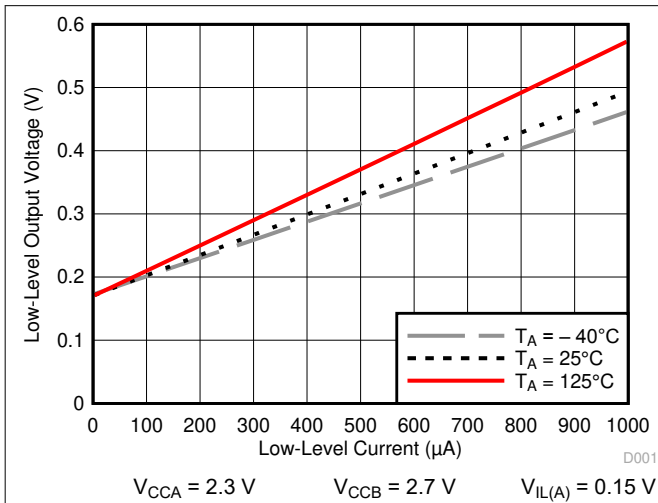
Figure 7-1. Low-Level Output Voltage ( V_{OL(Bx)} ) vs Low-Level Current ( I_{OL(Bx)} )
