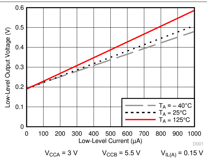
Figure 7-2. Low-Level Output Voltage ( V_{OL(Bx)} ) vs Low-Level Current ( I_{OL(Bx)} )
