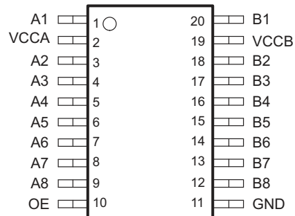
Figure 5-1. PW PACKAGE 20-PIN TSSOP (TOP VIEW)
