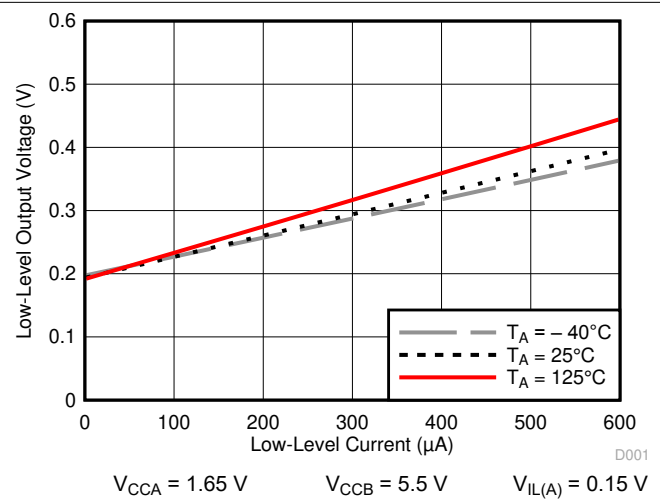
Figure 7-4. Low-Level Output Voltage ( V_{OL(Bx)} ) vs Low-Level Current ( I_{OL(Bx)} )
