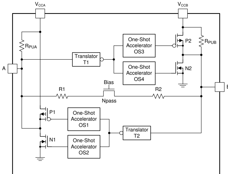
Figure 9-2. Architecture of a TXS0108E-Q1 Cell
