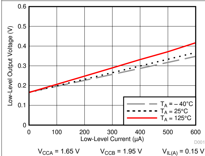
Figure 7-3. Low-Level Output Voltage ( V_{OL(Bx)} ) vs Low-Level Current ( I_{OL(Bx)} )
