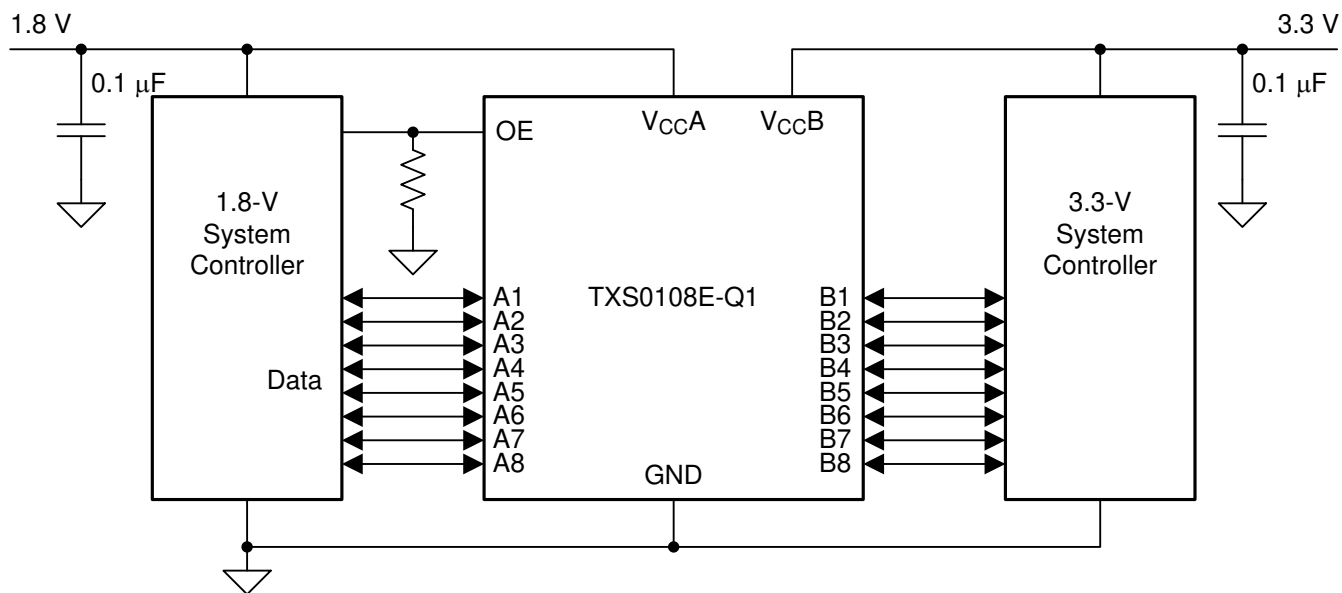
Figure 10-1. Typical Application Circuit
