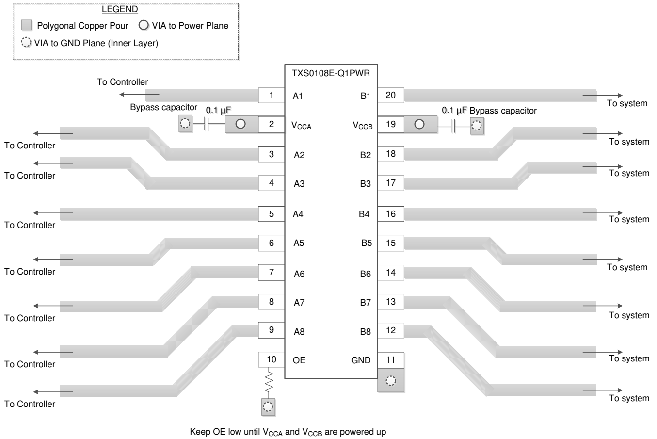
Figure 10-3. Layout Example
