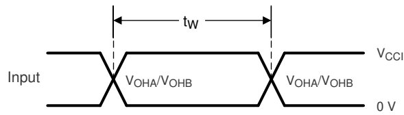
Figure 8-4. Pulse Duration (Push-Pull)
