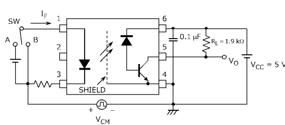
Fig. 13.1.6 Common-Mode Transient Immunity Test Circuit and Waveform
