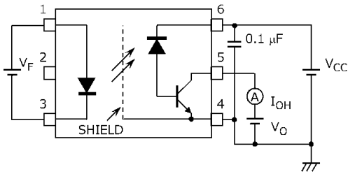
Fig. 13.1.1 IOH Test Circuit
