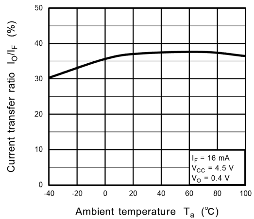
Fig. 13.2.6 I_O / I_F - T_a
