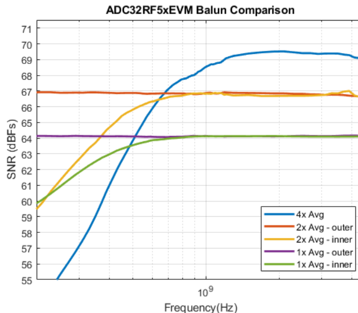
Figure 5-1. Balun Comparison
