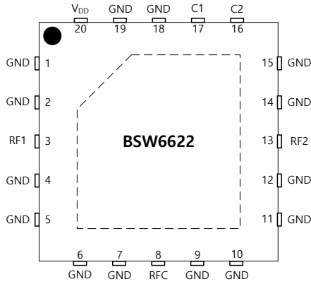
Figure 3. Pin Description
