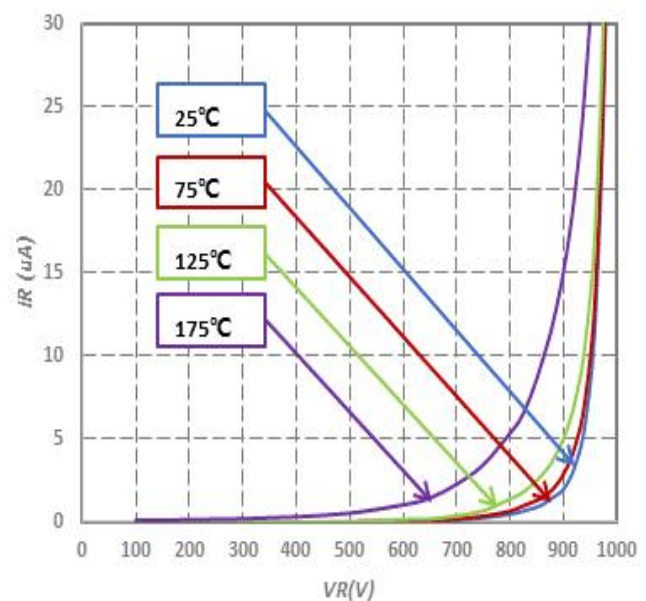
Fig.2-Typical Reverse Characteristics
