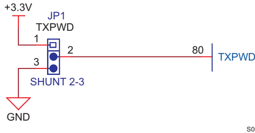
Figure 2. TXPWD Header JP1 Schematic
