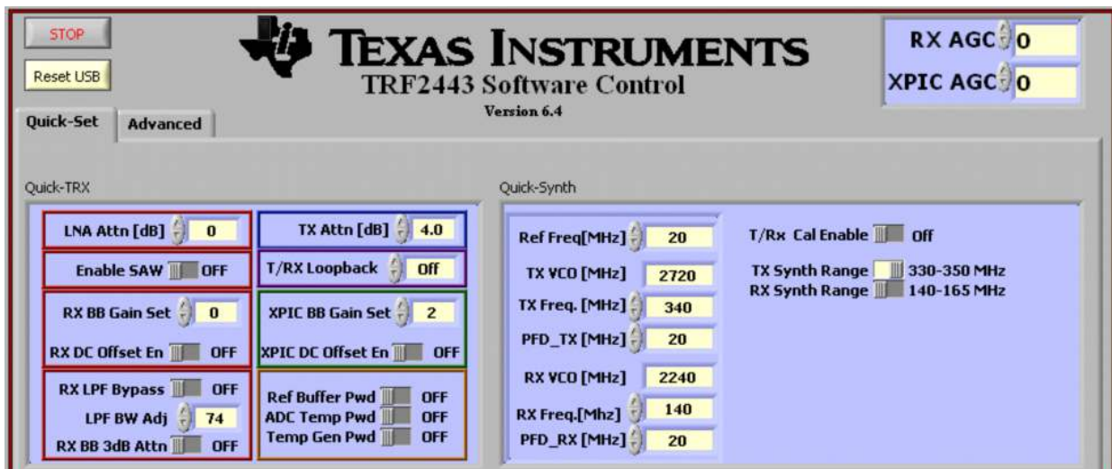
Figure 32. XPIC Receiver Min Gain GUI
