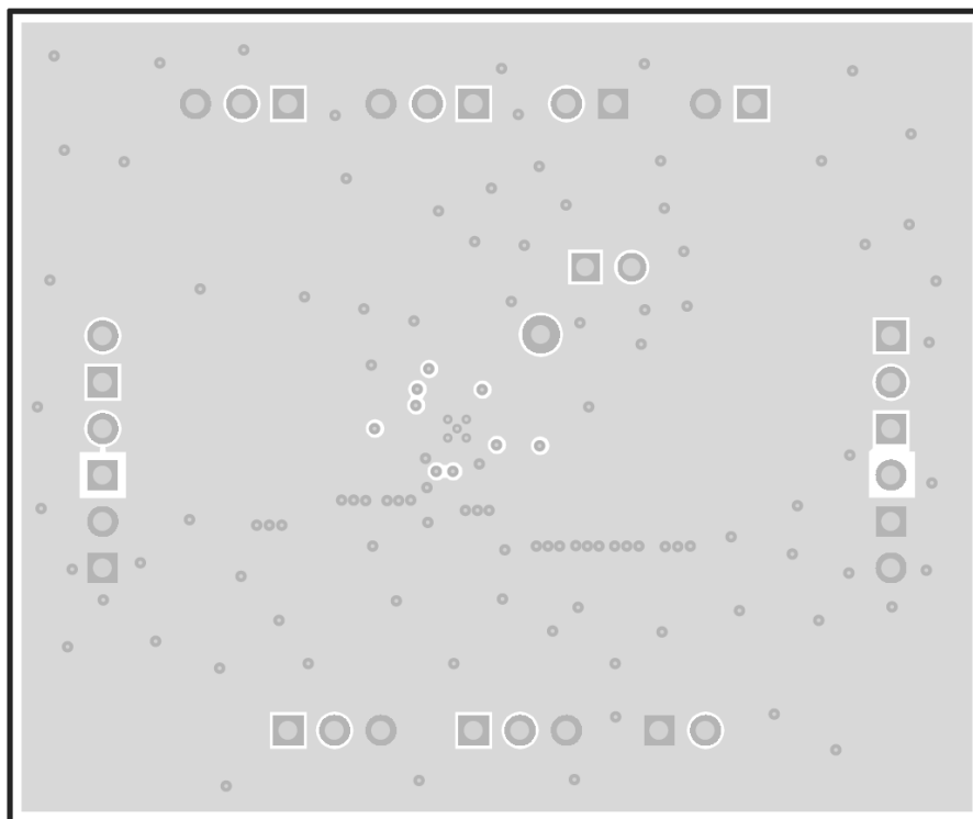
Figure 4-4. Internal Layer 1
