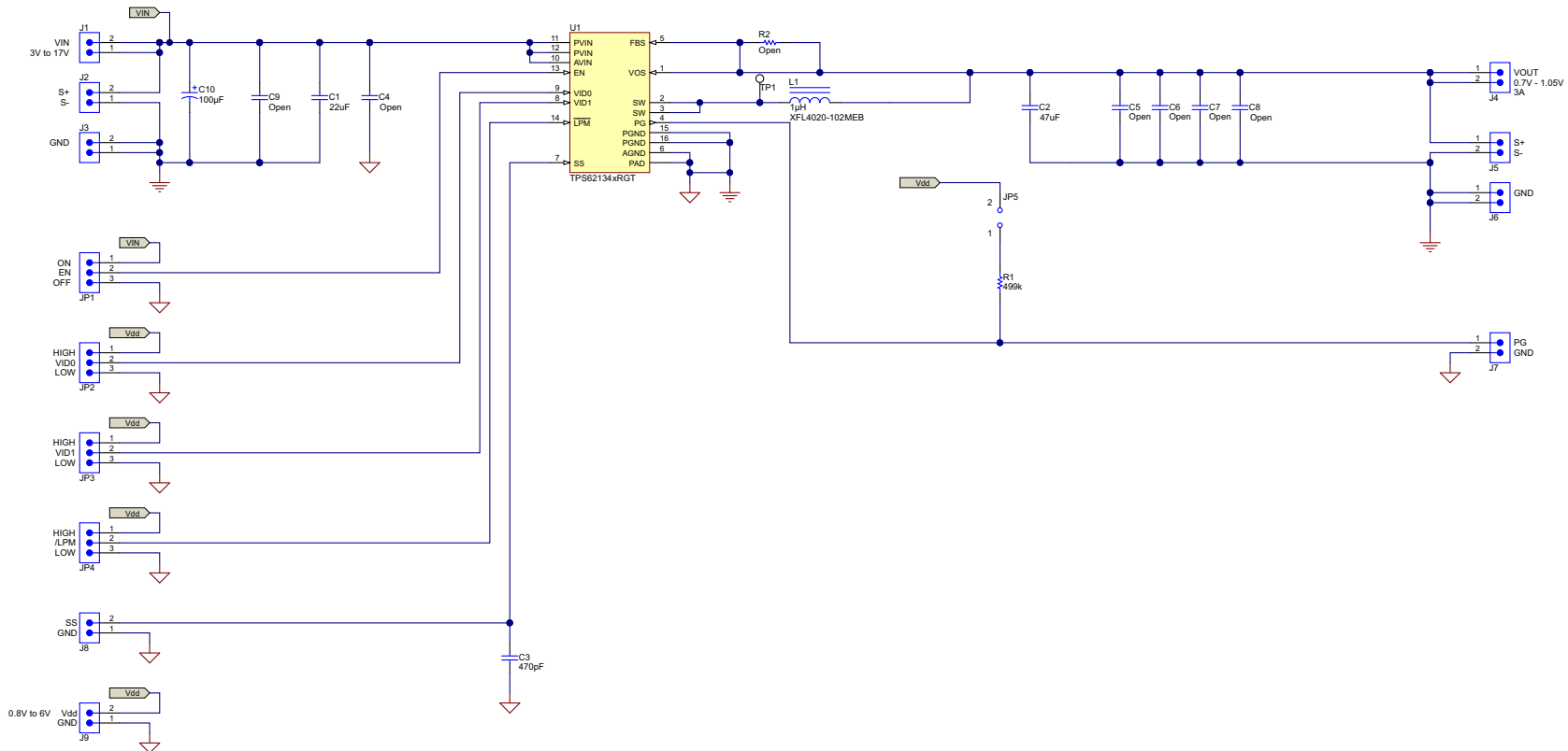
Figure 5-1. TPS62134xEVM-595 Schematic
