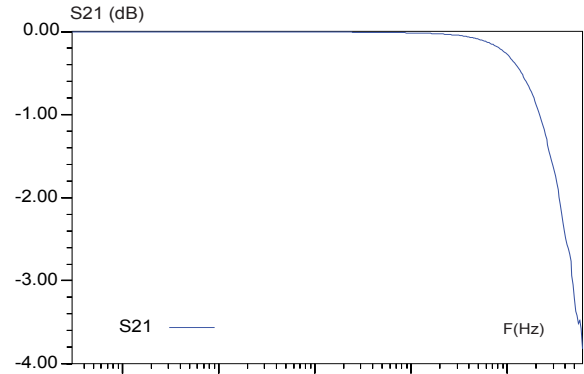
Figure 3. S21 attenuation measurement result
