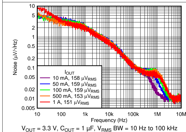
Figure 5. Output Spectral Noise Density
