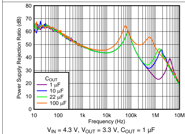
Figure 3. PSRR vs C_{OUT}
