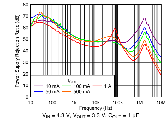
Figure 1. PSRR vs I_{OUT}
