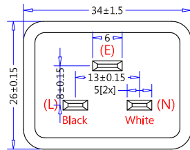
FM-320 (IEC 60320, C20, 20A 250V~) (Dimensions of Inlets Face)
