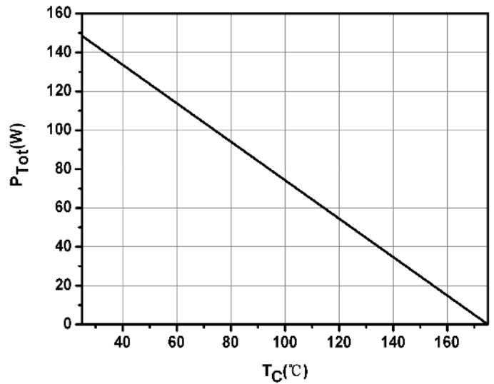
Fig.6-Power Derating
