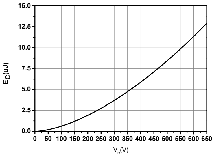
Fig.5-Capacitance Stored Energy
