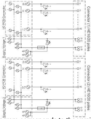
The wiring diagram corresponds to the version with LEDs.
