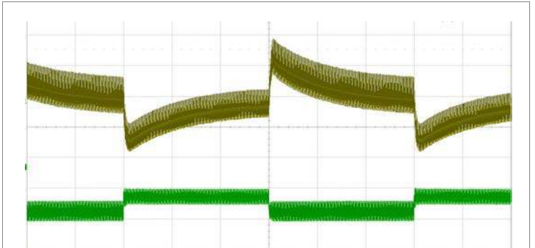
Output voltage response to load current step-change (0.475-0.7125-0.475 A) at: T_{PI} = +25^\circ\text{C} , V_i = 72\text{ V} . Top trace: output voltage (200mV/div.). Bottom trace: load current (500 mA/div.). Time scale: (500 \mu\text{s} /div.).
