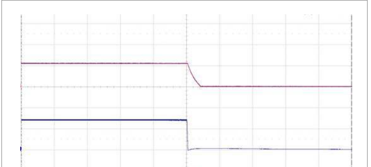
Shut-down enabled by disconnecting V_i at: T_{PI} = +25^\circ\text{C} , V_i = 72\text{ V} , I_o = 0.95\text{ A} resistive load. Top trace: output voltage (50 V/div.). Bottom trace: input voltage (50 V/div.). Time scale: (5 ms/div.).
