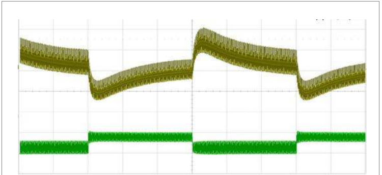
Output voltage response to load current step-change (0.525-0.7875-0.525 A) at: T_{PI} = +25^{\circ}C , V_I = 72 V . Top trace: output voltage (200mV/div). Bottom trace: load current (500m A/div). Time scale: (500 \mu s/div.).
