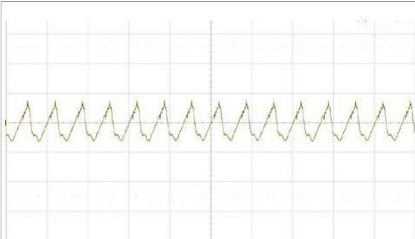
Output voltage ripple at: T_{PI} = +25^\circ\text{C} , V_i = 72\text{ V} , I_o = 0.95\text{ A} resistive load. Trace: output voltage (200 mV/div.). Time scale: (10 \mu\text{s} /div.). 20 MHz bandwidth.
