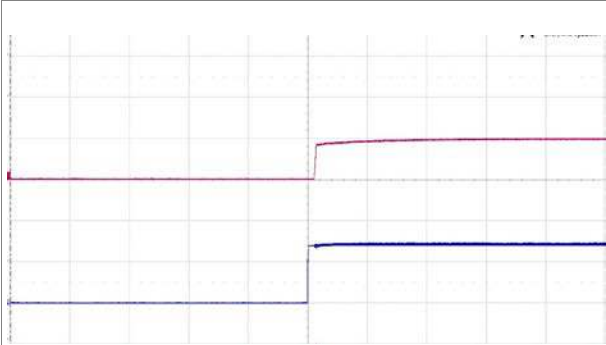
Start-up enabled by connecting V_I at: T_{PI} = +25^{\circ}C , V_I = 72 V , I_O = 1.05 A resistive load. Top trace: output voltage (50 V/div). Bottom trace: input voltage (50 V/div). Time scale: (50 ms/div.).
