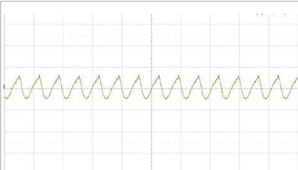
Output voltage ripple at: T_{PI} = +25^{\circ}C , V_I = 72 V , I_O = 1.05 A resistive load. Trace: output voltage (200 mV/div). Time scale: (10 \mu s/div.). 20 MHz bandwidth.
