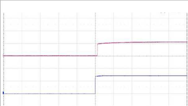
Start-up enabled by connecting V_i at: T_{PI} = +25^\circ\text{C} , V_i = 72\text{ V} , I_o = 0.95\text{ A} resistive load. Top trace: output voltage (50 V/div.). Bottom trace: input voltage (50 V/div.). Time scale: (50 ms/div.).
