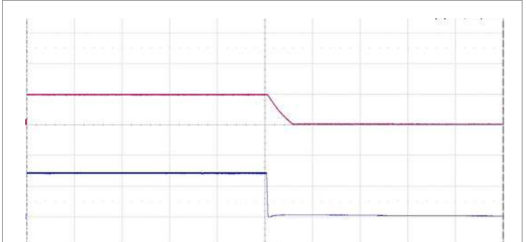
Shut-down enabled by disconnecting V_I at: T_{PI} = +25^{\circ}C , V_I = 110 V , I_O = 1.05 A resistive load. Top trace: output voltage (50 V/div). Bottom trace: input voltage (50 V/div). Time scale: (5 ms/div.).
