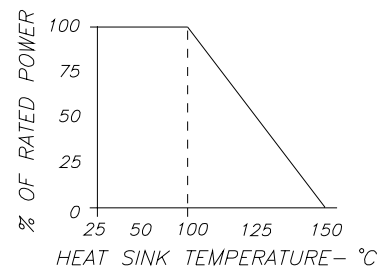
DERATING CURVE:
