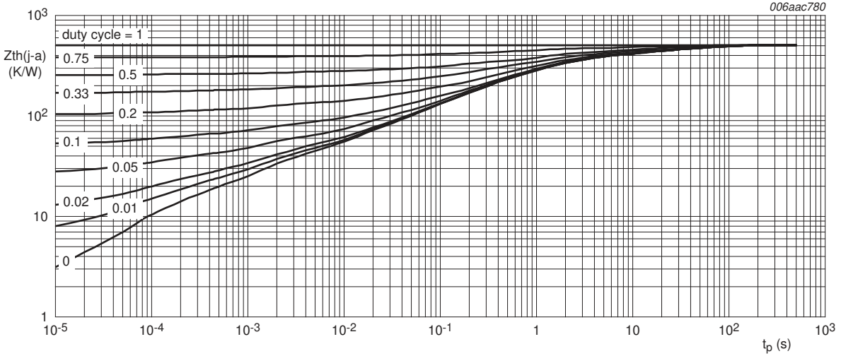
Fig 5. Transient thermal impedance from junction to ambient as a function of pulse duration for PDTC143ZU (SOT323); typical values
