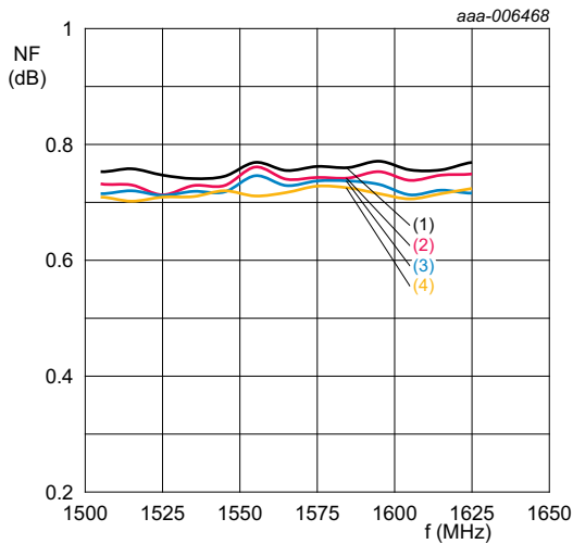
T_{\text{amb}} = 25 \text{ }^\circ\text{C}; no jammer, including PCB losses. (1) V_{CC} = 1.5 \text{ V} (2) V_{CC} = 1.8 \text{ V} (3) V_{CC} = 2.85 \text{ V} (4) V_{CC} = 3.1 \text{ V}
