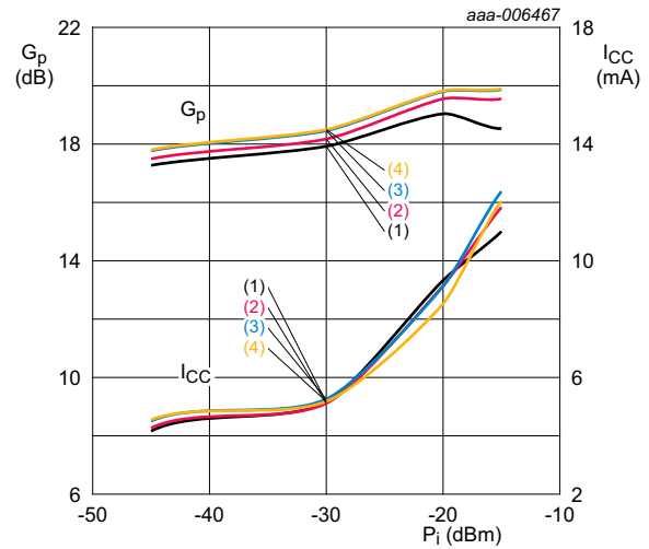
f = 1575 \text{ MHz}; T_{\text{amb}} = 25 \text{ }^\circ\text{C}. (1) V_{CC} = 1.5 \text{ V} (2) V_{CC} = 1.8 \text{ V} (3) V_{CC} = 2.85 \text{ V} (4) V_{CC} = 3.1 \text{ V}
