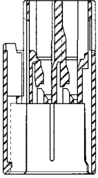
SECT. A-A
