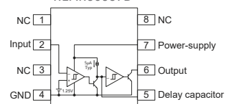
Voltage Detector (Reset-IC) REAR56957B
