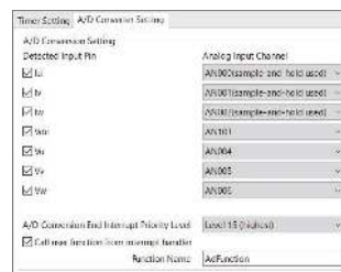
12-Bit A/D Converter (S12AD) Settings
