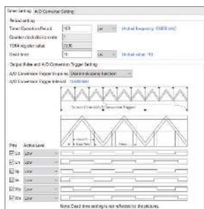
Timer (MTU/GPT) Settings
