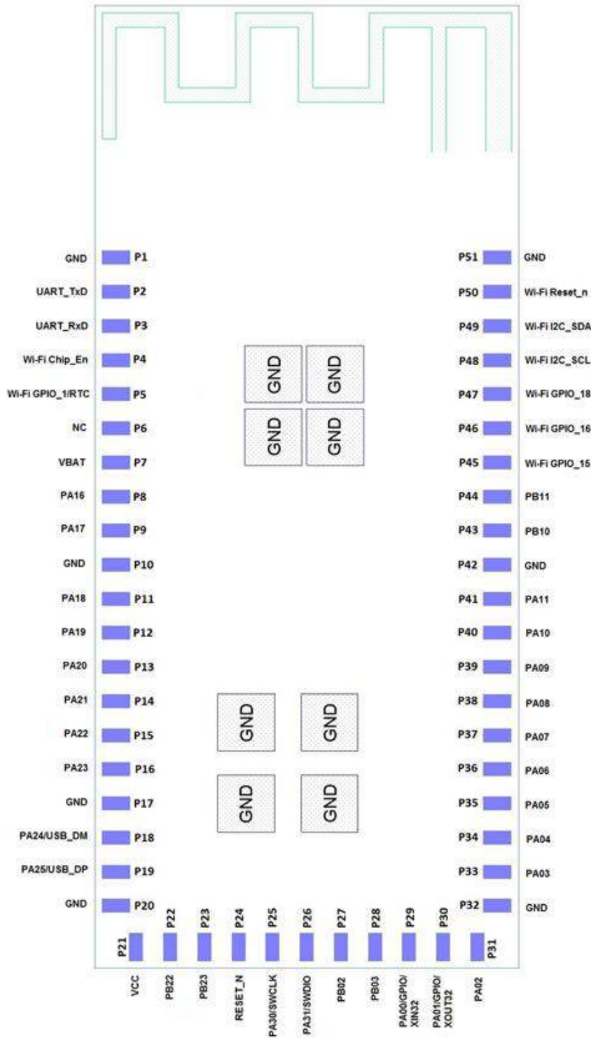
Figure 3-1. Pin Assignment
