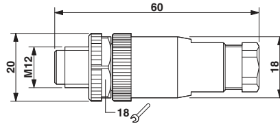
Dimensional drawing
