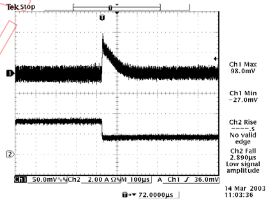
Transients 100% to 50% load 5.0 Vdc output
