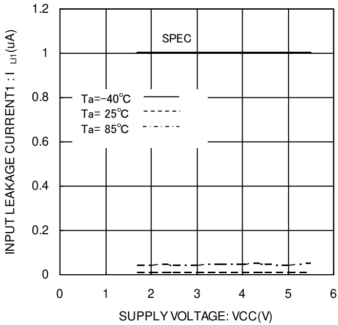
Figure 12. Input leakage current I_{LI}(DI)
