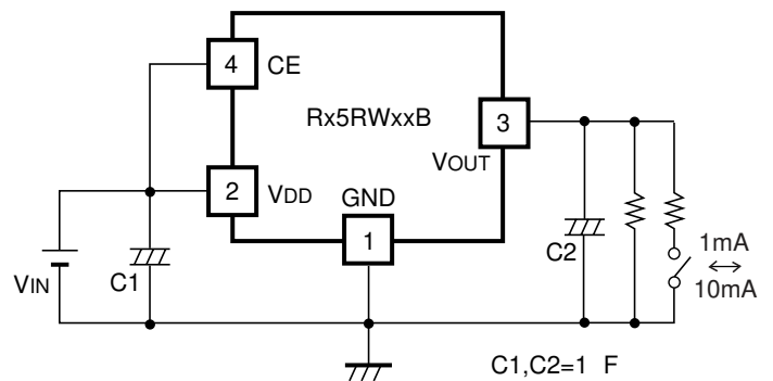
Load Transient Response Test Circuit
