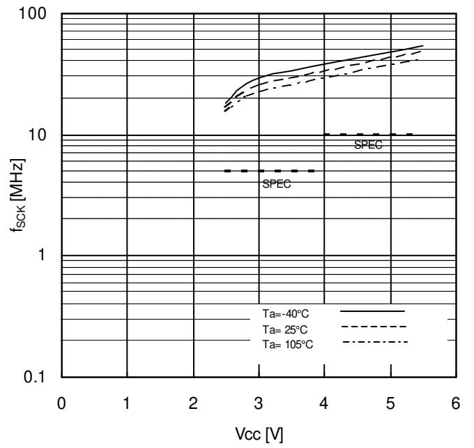
Figure 14. SCK frequency vs Supply Voltage
