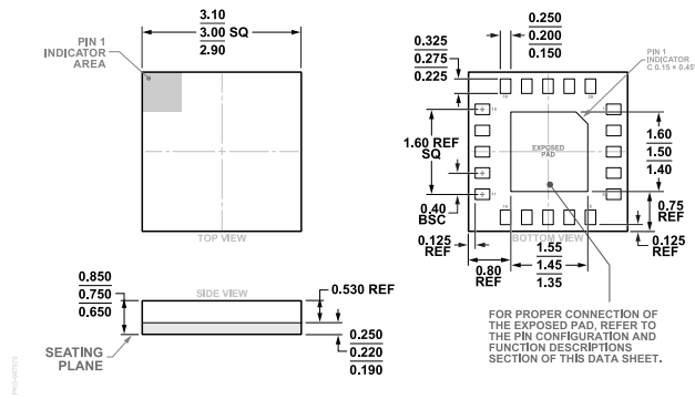
Figure 18. 20-Terminal Land Grid Array [LGA] 3 mm x 3 mm Body and 0.75 mm Package Height (CC-20-17) Dimensions Shown in Millimeters
