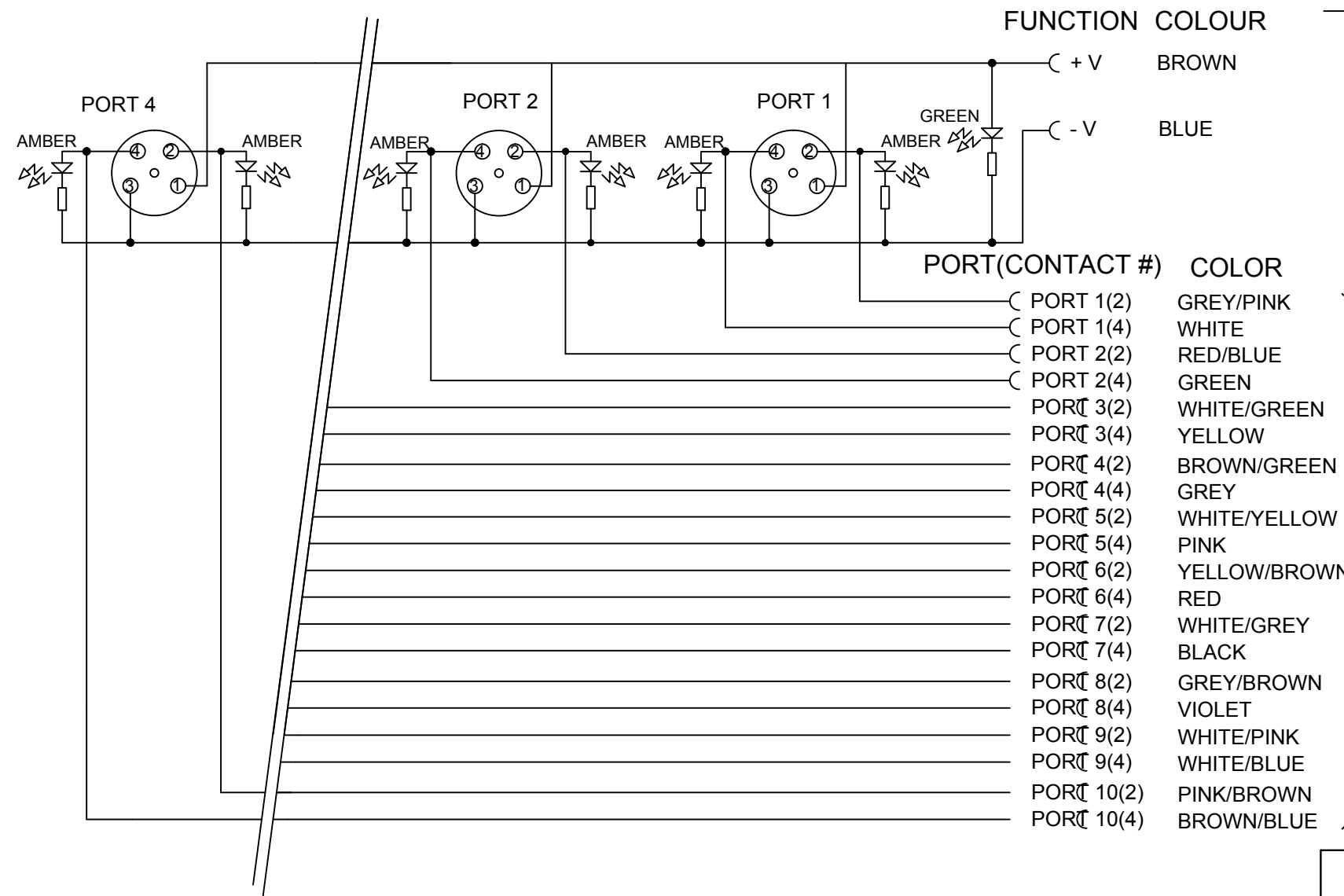
WIRING DIAGRAM
