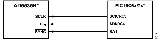
Figure 18. AD5535B-to-PIC16C6x/7x Interface
