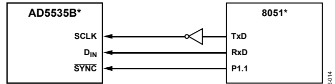
Figure 19. AD5535B-to-8051 Interface
