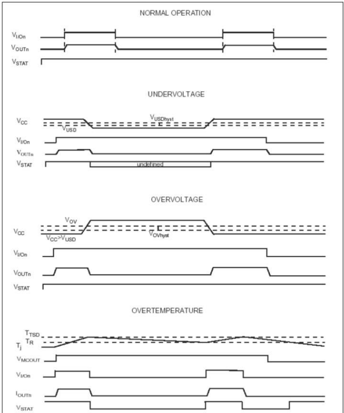
Figure 6. Waveforms
