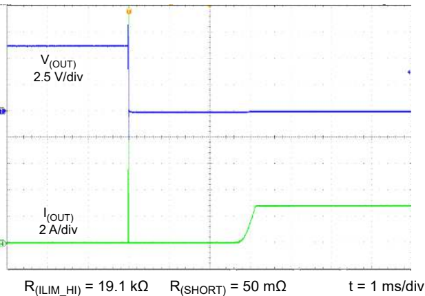
Figure 6-26. Hot Short
