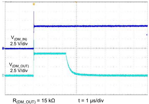
Figure 6-29. DM_IN Short to V_{BUS} Response Time
