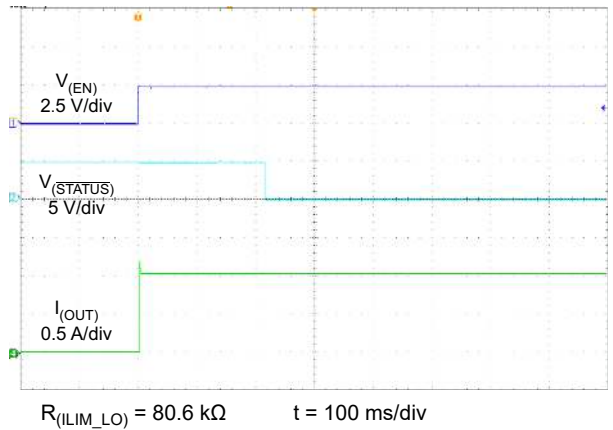
Figure 6-27. Load-Detection Set Time
