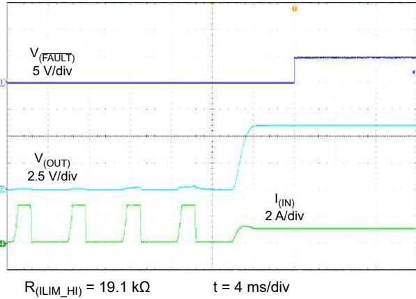
Figure 6-24. Short-Circuit to Full-Load Recovery
