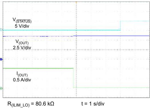
Figure 6-28. Load Detection Reset Time
