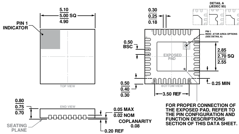
Figure 27. 32-Lead Lead Frame Chip Scale Package [LFCSPP] 5 mm × 5 mm Body and 0.75 mm Package Height (CP-32-21)
