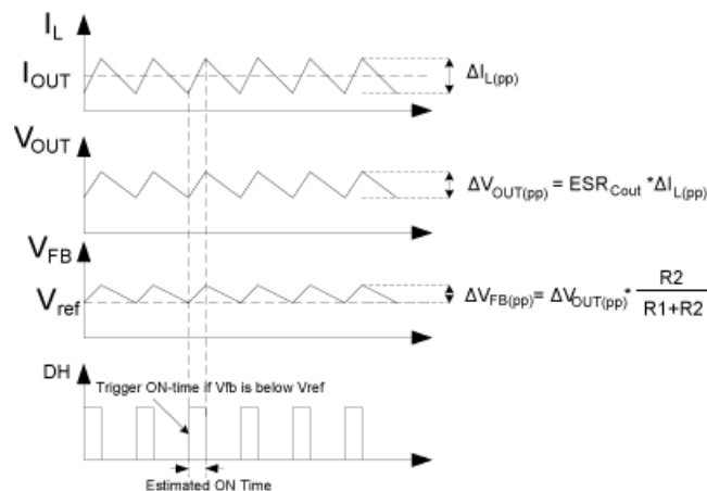
Figure 2. MIC26600 Control Loop Timing
