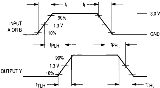
Figure 1. Switching Waveforms
