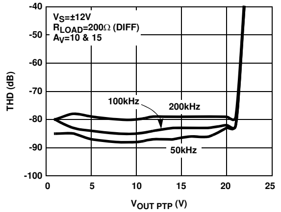
FIGURE 8. DISTORTION RESULTS
