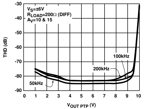
FIGURE 10. DISTORTION RESULTS
