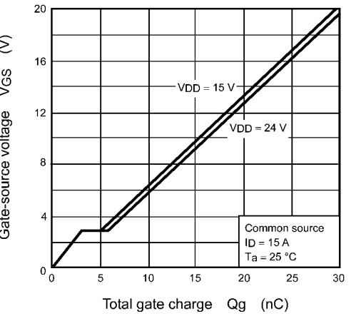
Fig. 7.11 Dynamic Input Characteristics
