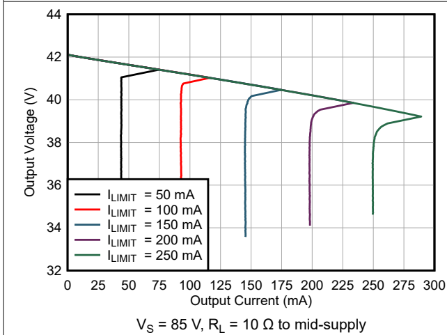
Figure 6-33. Output Voltage vs Output Sourcing Current
