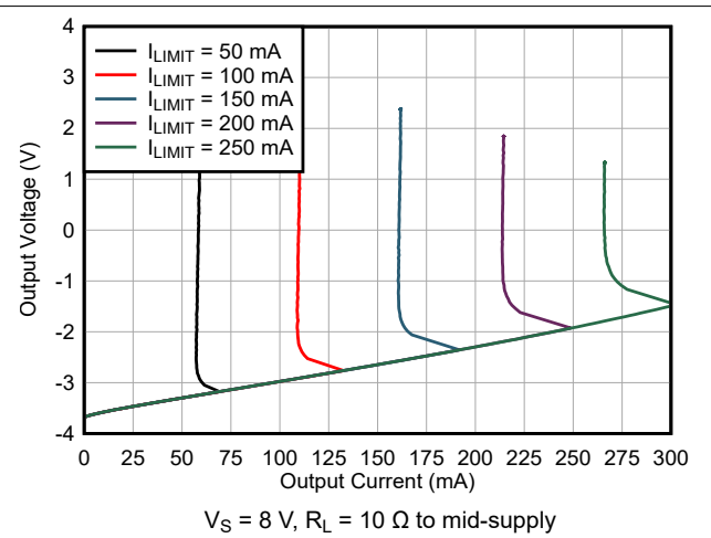
Figure 6-32. Output Voltage vs Current Limit Set
