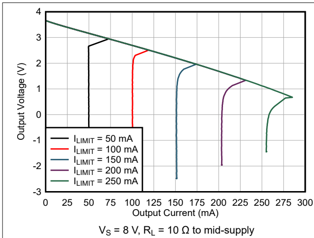
Figure 6-31. Output Voltage vs Current Limit Set
