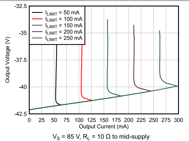
Figure 6-34. Output Voltage vs Output Sinking Current
