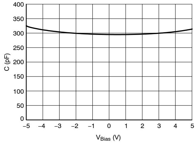
Figure 7. CV Characteristics
