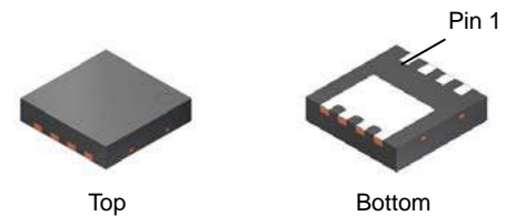
PQFN8 CASE 483AX
