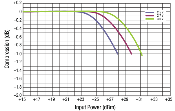
Figure 8. Compression vs Input Power @ 5 to 6 GHz
