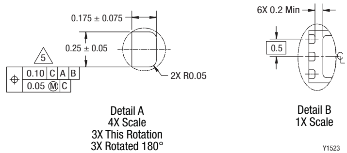
Figure 13. SKY13411-374LF 6-Pin QFN Package Dimensions
