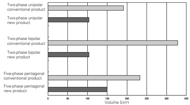
Figure 3 Size comparison
