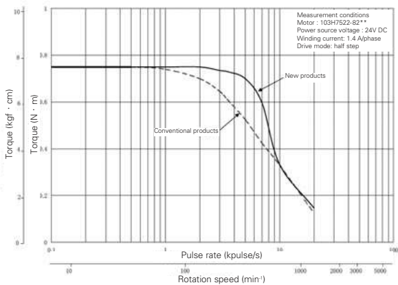
Figure 6 Frequency and torque characteristics
