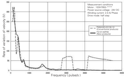
Figure 7 Vibration characteristics
