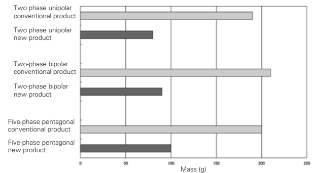
Figure 4 Weight comparison
