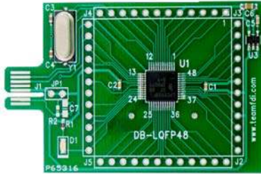
Board Dimensions 2.268" x 1.5"
