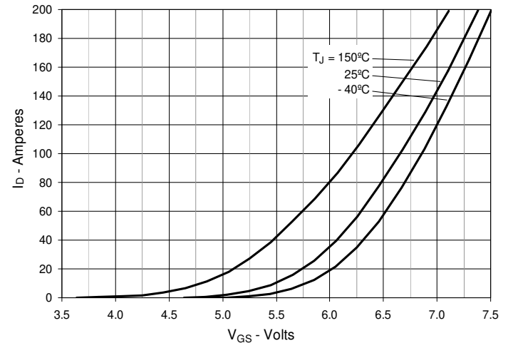
Fig. 6. Input Admittance
