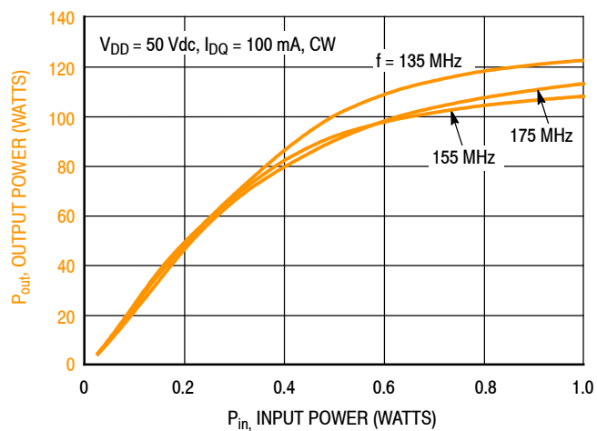
Figure 43. CW Output Power versus Input Power and Frequency
