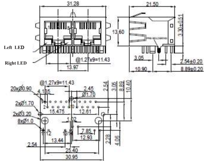
MB (1000 Base-T)
