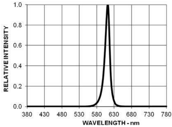
Figure 8: Relative Luminous intensity vs. Wavelength
