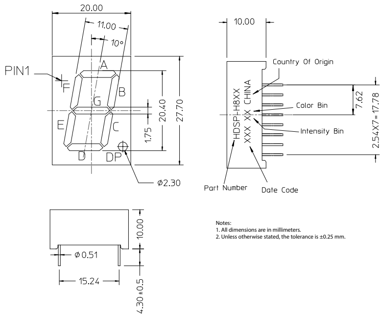
Figure 1: Package Dimension
