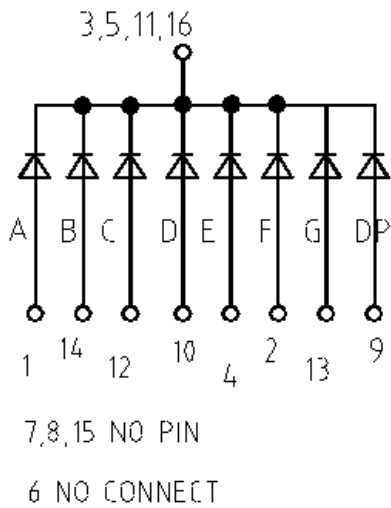
Figure 2: Circuit Diagram
