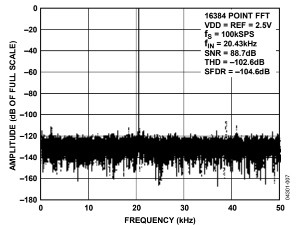
Figure 13. FFT Plot
