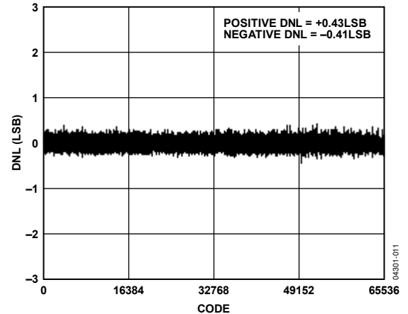
Figure 11. Differential Nonlinearity vs. Code
