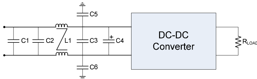
Figure 20. EMI Filter
