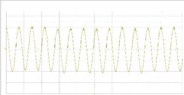
Output voltage ripple at: T_{P1} = +25^{\circ}\text{C} , V_i = 110\text{ V} , I_o = 0.625\text{ A} resistive load. Trace: output voltage (20 mV/div.). Time scale: (5 μs/div.). 20MHz bandwidth
