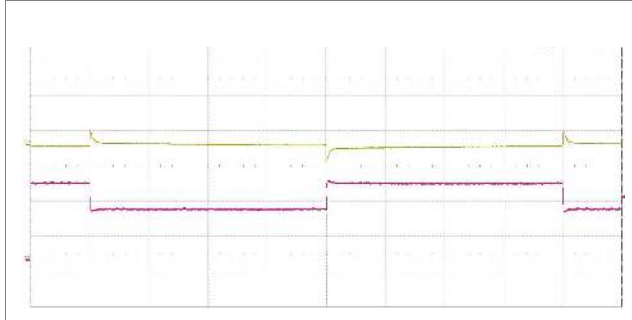
Output voltage response to load current step-change (0.312-0.468-0.312 A) at: T_{P1} = +25^{\circ}\text{C} , V_i = 110\text{ V} . Top trace: output voltage (500 mV/div.). Bottom trace: load current (200 mA/div.). Time scale: (2 ms/div.).
