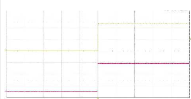
Start-up enabled by connecting V_i at: T_{P1} = +25^{\circ}\text{C} , V_i = 110\text{ V} , I_o = 0.625\text{ A} resistive load. Top trace: output voltage (20 V/div.). Bottom trace: input voltage (50 V/div.). Time scale: (200 ms/div.).
