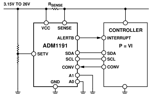
Figure 2. Applications Diagram
