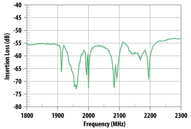
Figure 4. Tx-Rx Isolation
